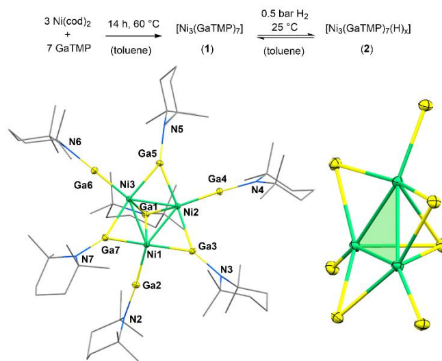
Figure 2. Above: Reaction scheme of the cluster synthesis of 1 and the conversion by H 2 addition to yield the (poly-)hydride species 2 . – Below: The molecular structure of 1 in the solid-state is shown left (thermal ellipsoids are given at the 50% probability level). TMP ligands are given in wireframe depiction and H atoms are omitted for clarity. Selected bond length (Å) and angle (deg) ranges: Ni-Ni 2.383 - 2.396, Ni-μ 2 -Ga 2.175 - 2.184, Ni-μ 2 -Ga 2.214 - 2.227, Ni-μ 3 -Ga 2.314 - 2.411; Ni-Ni-Ni 59.7° - 60.3°. The Ni/Ga metal core structure of 1 is shown at the right side. TMP ligands are omitted. Green plane highlights the well-accessible Ni 3 triangle.
