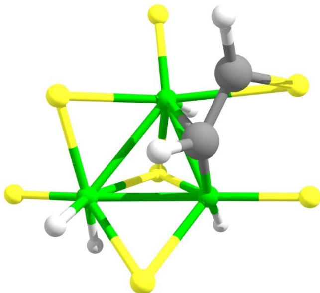
Figure 5. DFT-optimized geometry of the 2_{\text{Tetra}}-(\text{C}_2\text{H}_2) adduct, which shows pronounced Ga-C interactions.
