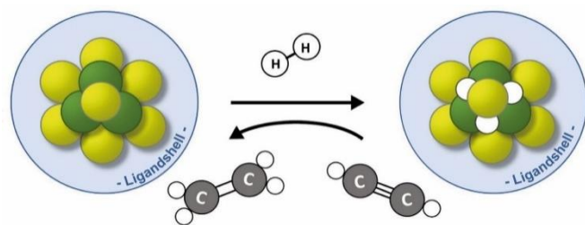
Figure 1. Conceptual scheme depicting the reaction of the alkylamide ligand protected cluster [Ni 3 (GaTMP) 7 ] ( 1 , left) with H 2 to yield the (poly-)hydride clusters [Ni 3 (GaTMP) 7 (H) x ] ( 2 , right; x = 2,4,6). Color code: yellow, Ga; green Ni; white, H; blue, TMP ligand shell (TMP = 2,2,6,6-tetramethylpiperidiny). The (poly-)hydride clusters 2 (right) enable catalytic semihydrogenation of alkynes to alkenes. The structures of 1 and 2 may serve as a molecular model for the catalytically active sites at the surface of the Ni 5 Ga 3 solid-state phase.
