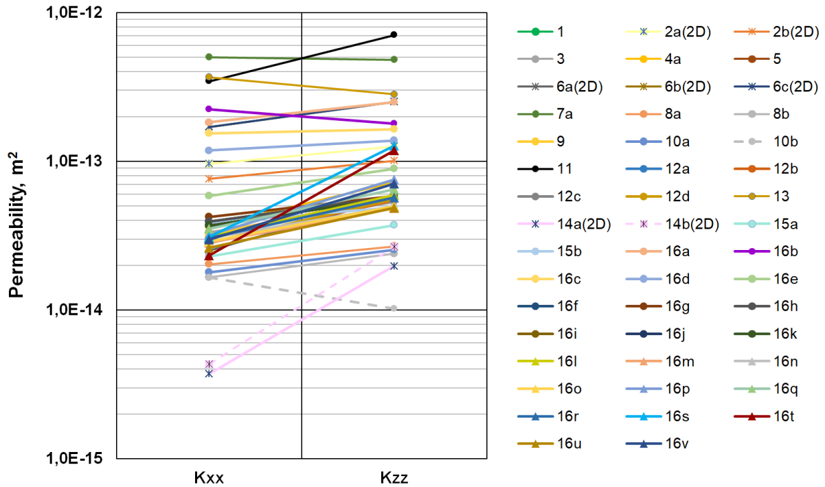
Figure 13: Transverse permeability K_{xx} and K_{zz} results (without analytically predicted ones). 2D computations are marked by 'x'
