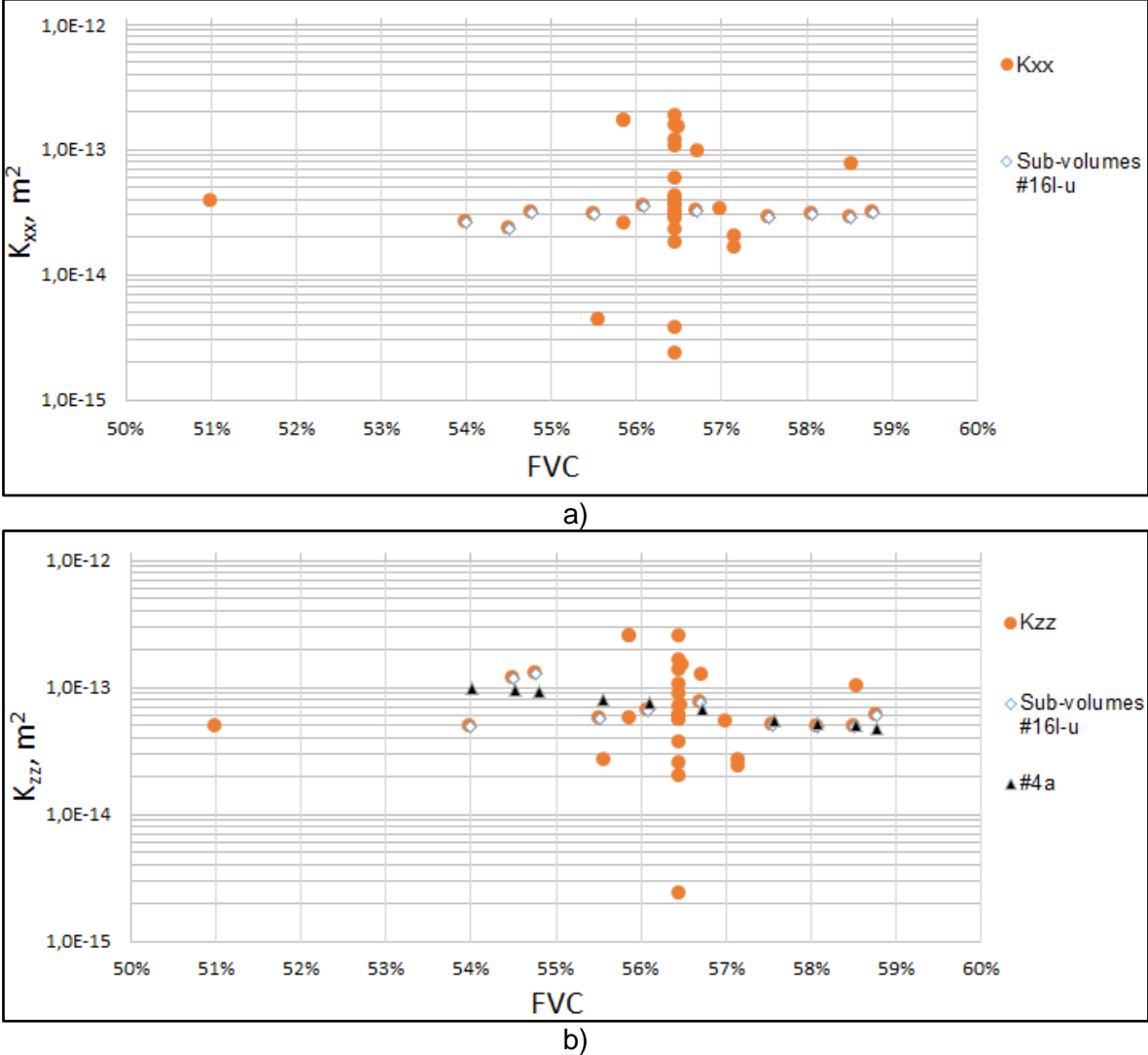
Figure 16: Correlation between the fiber volume fraction and predicted transverse permeability a) K_{xx} ; b) K_{zz} (without excluded results #7a, #11, #13, #16b)
