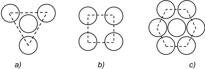
Figure 5: Idealized types of fiber packing assumed in analytical models: a) triangular; b)quadratic; c) hexagonal
