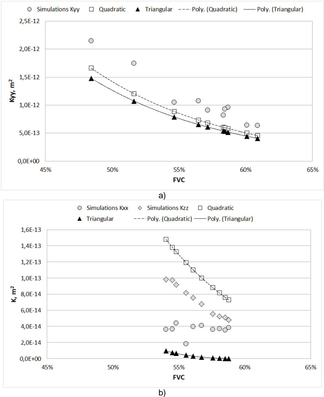
Figure 7: Comparison on 10 sub-volumes of the numerical results #4 and analytically predicted values with the corresponding FVC, fibers diameter of 9 μm, and assumptions of quadratic [15] or triangular [17] fiber packing
