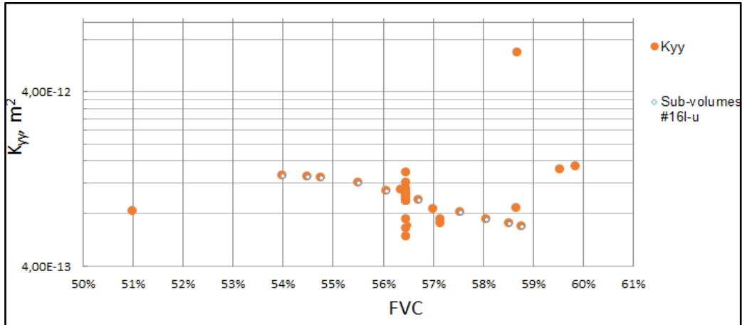
Figure 5: Correlation between the predicted axial permeability and fiber volume fraction
