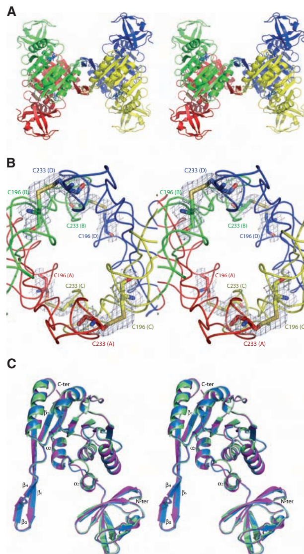
Figure 1. Overall organization of Pab TrmI (Stereoviews). (A) Pab TrmI tetramer structure in complex with SAH. Subunits A and B, colored red and green, respectively, form one tight dimer and subunits C and D, colored yellow and blue, respectively, form another one. SAH is shown in blue sticks. (B) Detail of the four inter-monomer disulfide bonds that stabilize the Pab TrmI tetramer. A 2 Fobs-Fcalc electron density map contoured at the level of one standard deviation is superimposed on the structure. (C) Superposition of one Pab TrmI monomer from Crystal form I (in magenta), Crystal Form II (in blue) and Crystal Form III (in green).
