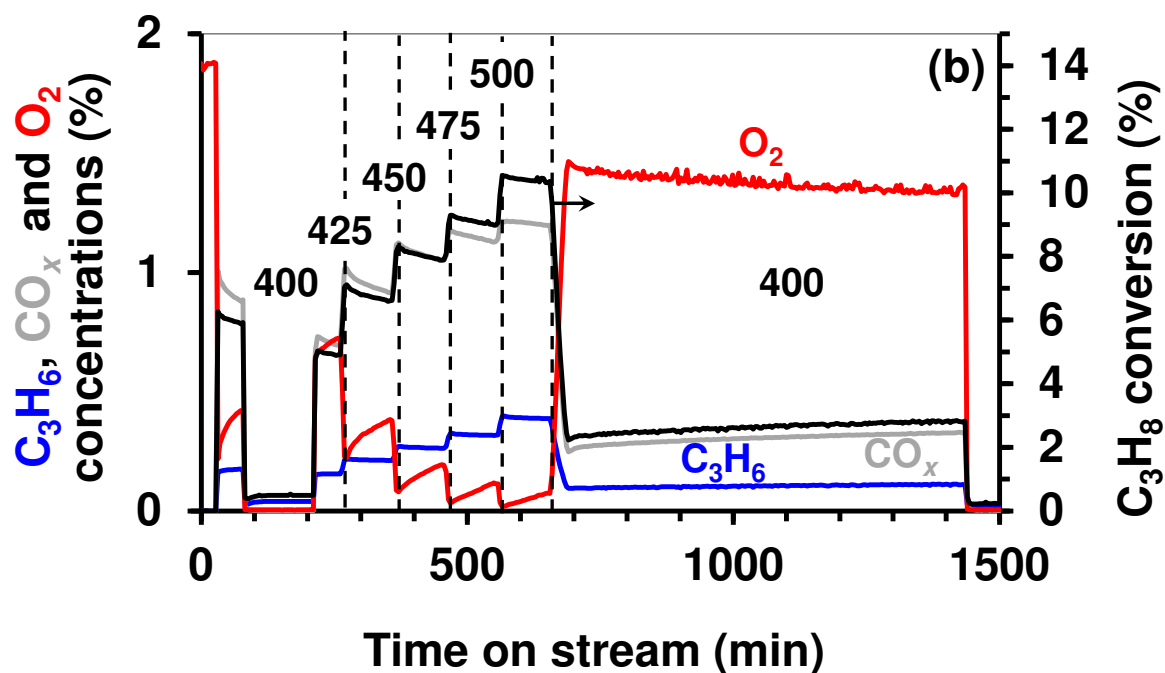
Figure S6. Influence of the removal of O 2 from a 8.2% C 3 H 8 (8.2%) – O 2 (1.9%) – He feed at 400 °C after ODHP reaction from 400 to 500 °C on (a) Co 3.0 -Siβ-pH-2.5 and (b) Co 3.1 -Siβ-pH-
