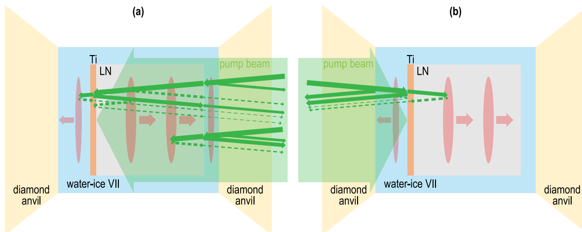
Fig. 2. Schematics of the pump and probe light paths in our TDBS experiments on a single crystal of \text{LiNbO}_3 (LN) covered on one side with the thin Ti optoacoustic transducer and surrounded by water-ice VII in a DAC. The pump and probe laser beams are incident through a diamond anvil and a water ice layer on the same side of the sample. However, the experiments can be conducted from both sides of the sample, i.e. , from the LN side (a) and from the Ti side (b). Dashed lines indicate weakly scattered probe light by CAPs that are depicted as semitransparent red ellipses. Solid lines indicate the incident pump and probe beams, as well as much stronger reflections of the probe light by stationary interfaces of the sample. We present optical paths of only the strongest reflected probe rays, which can interfere with the acoustically-scattered light and made detectable contributions to the TDBS signals in our experiments (Section 3.2). We also present only those scatterings of the probe light by CAPs which contributions to the TDBS signals were revealed in our experiments.
