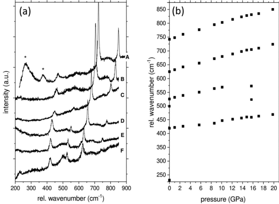
Figure 2. (a) Raman spectra of \gamma -Sn 3 N 4 synthesized at high pressures via a reaction of tin with molecular nitrogen in a LH-DAC. A - Spectrum of the sample synthesised at 20 GPa showed, in addition to two broad peaks of the nitrogen pressure medium at \omega=265 cm -1 and \omega=375 cm -1 (stars), three strong and narrow Raman peaks as well as three weak and broad ones belonging to \gamma -Sn 3 N 4 . (B-F) Evolution of the Raman spectra of \gamma -Sn 3 N 4 with pressure at RT. The spectra B, C, D, E, and F were measured at 15.7 GPa, 10.1 GPa, 5.7 GPa, 1.0 GPa, and 1 atm., respectively. (b) Pressure dependences of the Raman-band frequencies of \gamma -Sn 3 N 4 shown in (a).
