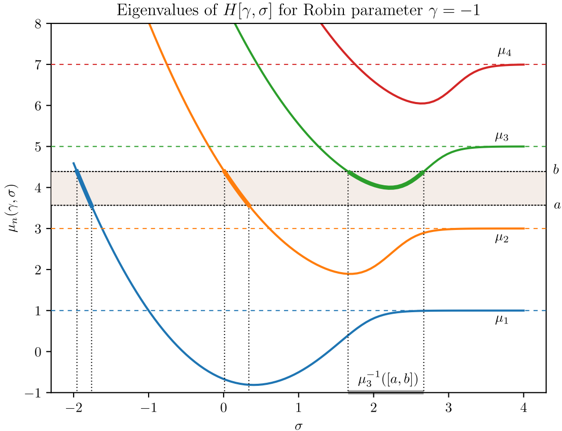
FIGURE 1. This figure shows the dispersion curves \mu_k(\gamma, \cdot) , for \gamma = -1 . We visualise the preimage of a given interval [a, b] \subset (2n - 3, 2n - 1) with n = 3 . The curves are obtained by a standard finite difference numerical scheme.
