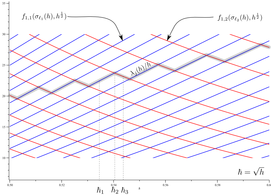
FIGURE 2. Illustration of the collection of semiclassical branches of eigenvalues. Here we plot the graphs of f_{1,q}(\sigma_\ell(h), h) with respect to the variable \hbar = \sqrt{h} , for q = 1 (blue curves) and q = 2 (red curves). The continuous curve of \lambda_j(h)/h , for fixed j , where \lambda_j(h) is the exact eigenvalue of \mathcal{L}_h , lies within the greyed stair-case like curve (of vertical width \mathcal{O}(h) ).
