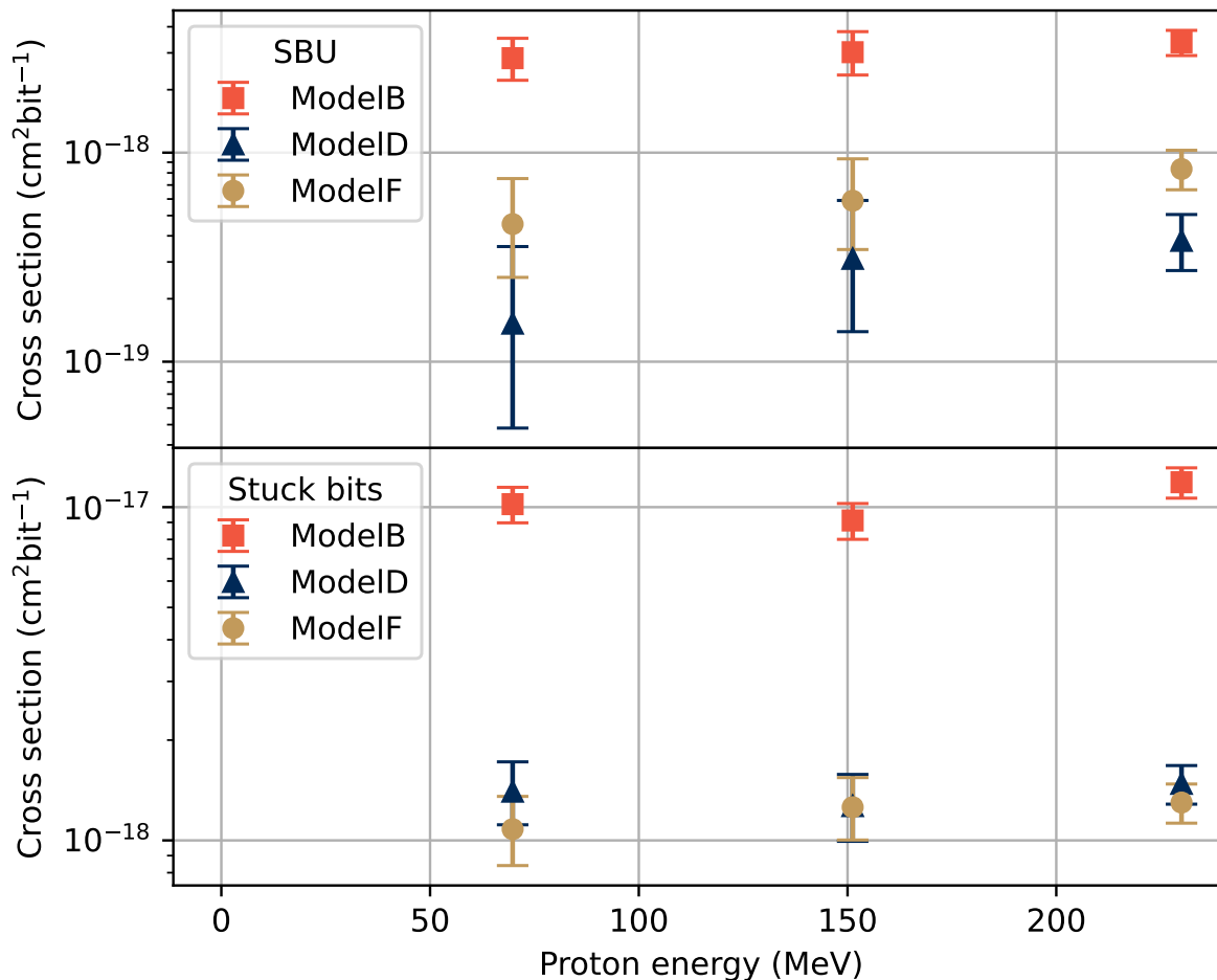
Fig. 5. Error cross sections for SBUs (top) and stuck bits (bottom) for the different memory parts, for the tested 128 Mib using a data refresh interval of 256 ms, thus larger cross sections than what can be expected for nominal operation using a 64 ms refresh interval. The events observed during static and dynamic tests have been combined in the figures, as well as the results from DUTs B1 and B2, D1 and D2, and F1 and F2.
