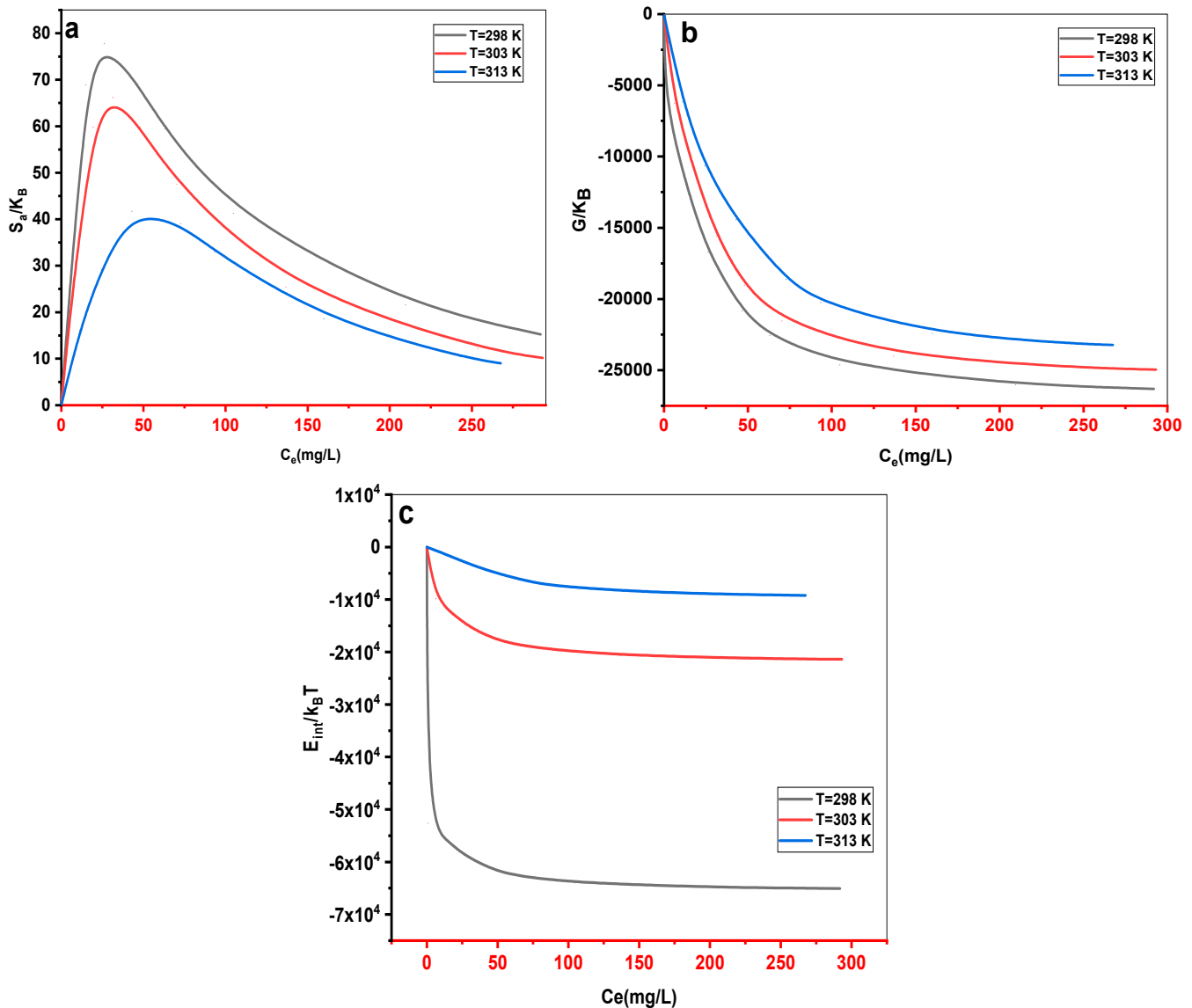
Figure 14. (a) Entropy, (b) free enthalpy, and (c) internal energy evolution as a function of concentration for MB adsorption by Cs adsorbent at various temperatures.
