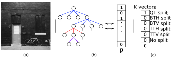
Fig. 5. Representation of our dataset. (a) is a luminance 64 \times 64 input block \mathbf{B} . (b) is the optimal partitioning of the block represented by a tree and transformed to the soft representation, i.e. a 480 elements vector \mathbf{p} . (c) is the hard representation, K vectors \mathbf{c} of 6 probabilities, that define the optimal split for each of the K blocks in the tree. K is the decision tree depth.
