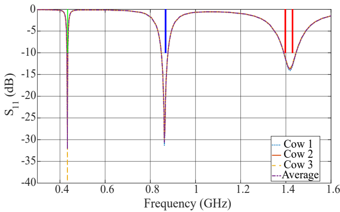
Fig. 5. Reflection coefficients of the conformal patch antenna simulated in a phantom with EM properties of cow's rumen fluid (3 cows and the average values in Table I). The green, blue, and red strips are the ISM bands at 434 MHz (433.05–434.79 MHz), 868 MHz (865–870 MHz), and 1400 MHz (1395–1400 MHz and 1427–1432 MHz), respectively.
