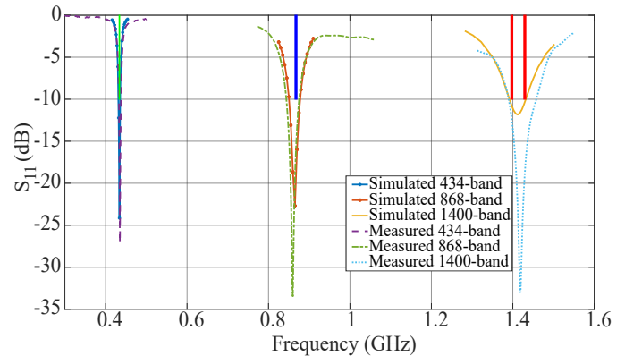
Fig. 9. Measured and simulated reflection coefficients |S_{11}| (dB) of the proposed antenna in the 200 mm \times \varnothing 300 mm cylindrical glass container filled with the liquid 1 for 434 MHz and 868 MHz and with liquid 2 for 1400 MHz. The green, blue, and red strips are the ISM bands at 434 MHz (433.05–434.79 MHz), 868 MHz (865–870 MHz), and 1400 MHz (1395–1400 MHz and 1427–1432 MHz), respectively.
