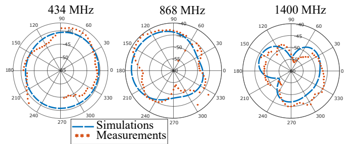
Fig. 11. Measured and simulated azimuthal gain (dBi) of the bolus antenna in the 200 \text{ mm} \times \varnothing 300 \text{ mm} cylindrical glass container filled with the liquid 1 for 434 MHz and 868 MHz and with liquid 2 for 1400 MHz.
