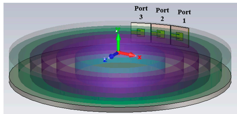
Figure 23. The simulation model of the plate Luneburg lens fed by three reduced size MPA with CSRR rotated to 90^\circ at z-axis.
