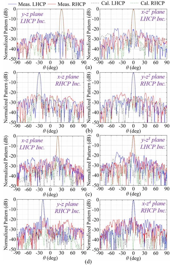
Fig. 12. Calculated and measured normalized CP radiation patterns of the TA antenna by exciting the K -band (a) LHCP and (b) RHCP feed arrays at 19.5 GHz, and the Ka -band (c) LHCP and (d) RHCP feed arrays at 29.5 GHz, where \hat{z}^1 = \hat{z}\cos 30^\circ + \hat{y}\sin 30^\circ , \hat{z}^2 = \hat{z}\cos 30^\circ - \hat{x}\sin 30^\circ , \hat{z}^3 = \hat{z}\cos 20^\circ - \hat{y}\sin 20^\circ , and \hat{z}^4 = \hat{z}\cos 20^\circ + \hat{x}\sin 20^\circ .
