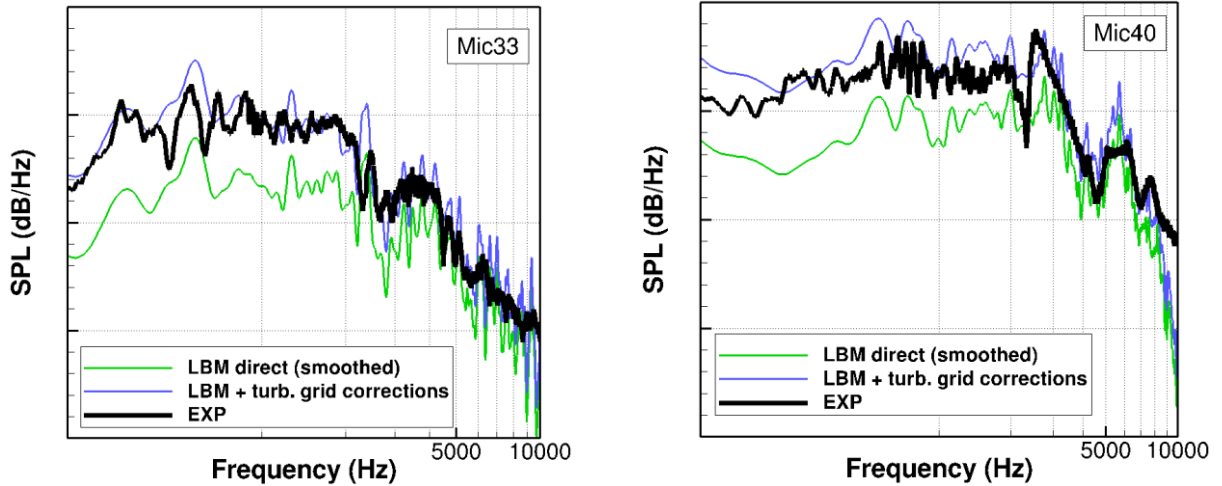
Figure 21. SPL comparisons on baseline case: direct LBM results (with and without correction) vs. experiment at Mach 0.34 for mic. 33 (left) and mic 40 (right) ; Log x-scale and 10 dB step between y-ticks.
