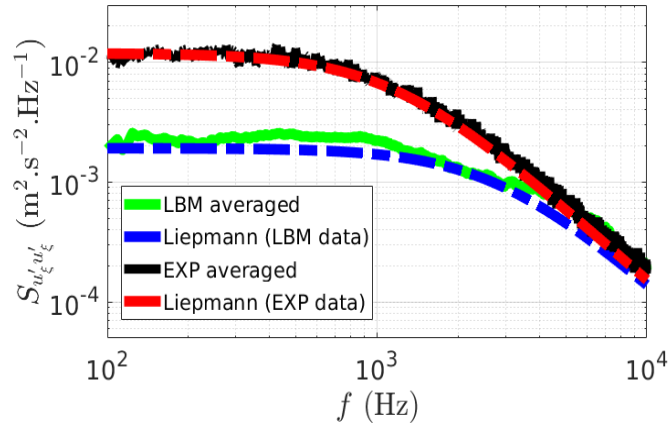
Figure 16. Turbulent velocity spectra of the axial velocity component obtained from LBM and comparisons with experiments.
