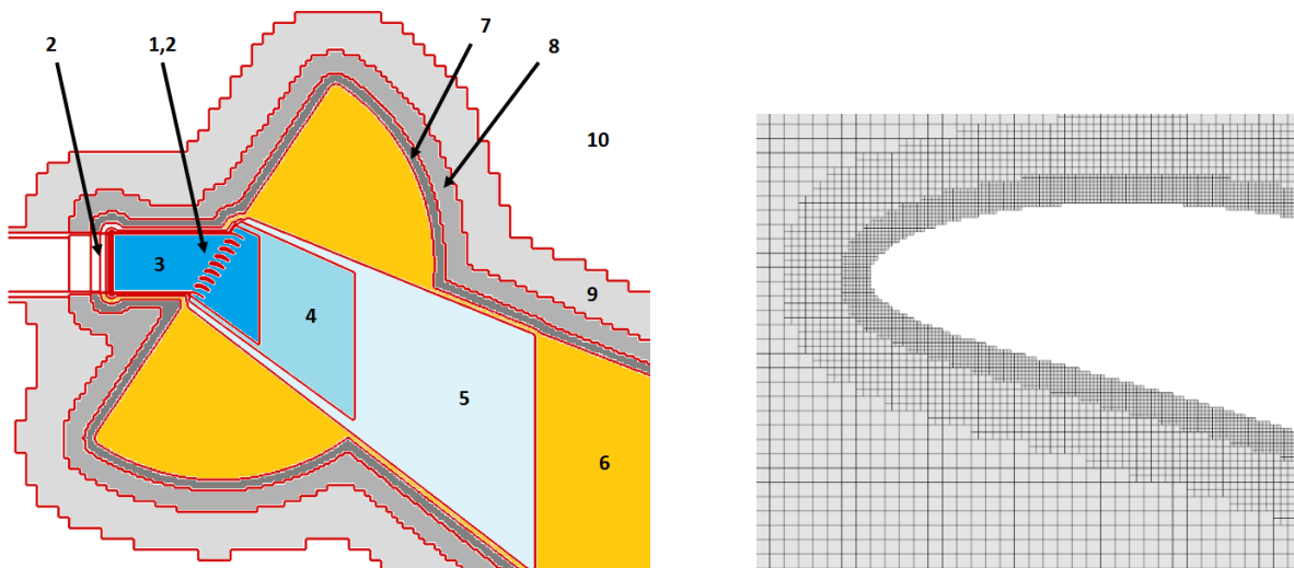
Figure 9. Mesh refinement levels in the plane z = 0 (left). Octree mesh for the "fine mesh" configuration around a NACA airfoil LE (right).
