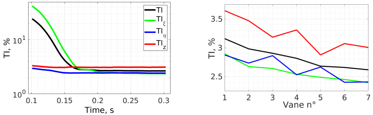
Figure 13. Temporal evolution of turbulence intensities using a moving average over 0.2 s (left). Converged turbulence intensities in front of each NACA airfoil (right).
