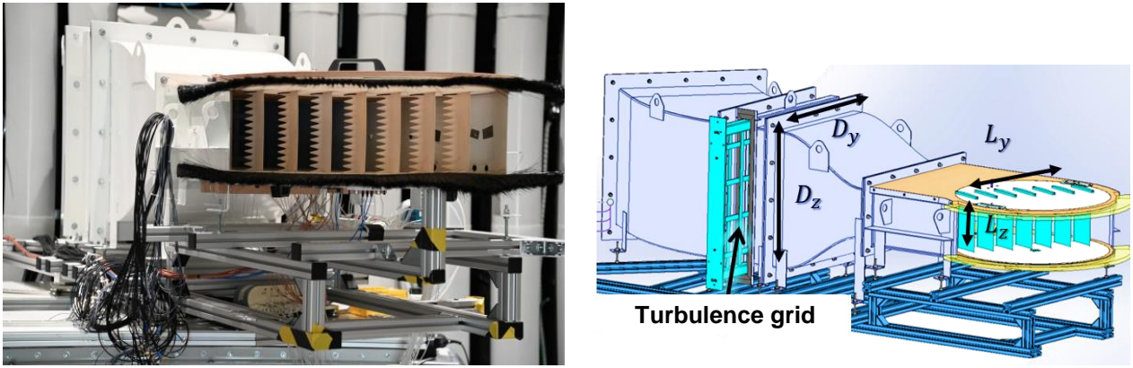
Figure 2. Picture of the cascade test rig (left). 3D geometric modeling of the bench with turbulence grid and vanes in cyan (right).
