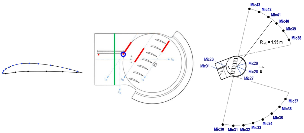
Figure 4. Pressure probes at the vane surface (left). Mid span cut of the geometry and wire probes locations (center). Far-field acoustic microphones (right).
