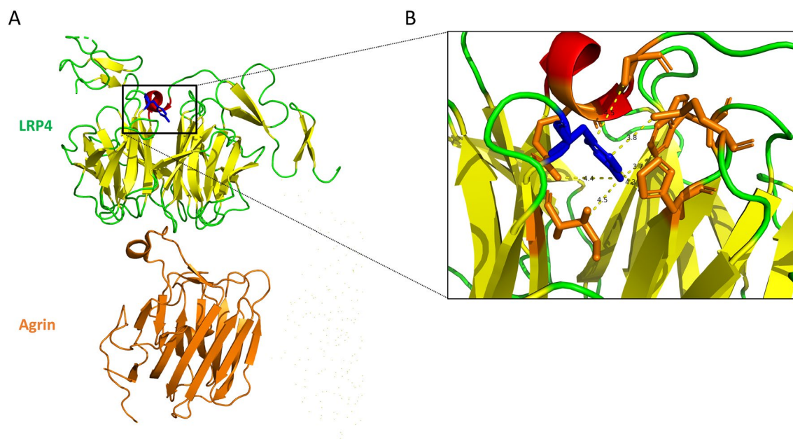
Figure 5. 3D view of \beta 1 propeller domain of LRP4 in complex with agrin involving Tyr607 mutation. (A) Backbone representation extracted from the crystal structure of LRP4, in complex with agrin (colored in orange), using PDB accession number 3V64. Tyr607 mutation is colored in blue. (B) Zoom view of the side chain interactions between Tyr607 (colored in blue) and neighbor residues (colored in orange). Inter side-chain distances lower than 5 Å are indicated by dash lines. For A and B figures were extracted from PyMol software.
