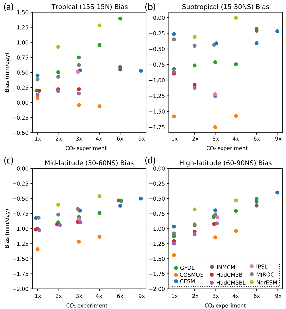
Figure 12. Zonally averaged model-data mean annual precipitation (MAP) bias for the (a) tropics (15°–15°N/S), (b) subtropics (15°–30°N/S), (c) mid latitudes (30°–60°N/S), and (d) high latitudes (60°–90°N/S). Panels (a–d) show the model-data bias in mm/day for the different model simulations, sorted by CO 2 forcing.
