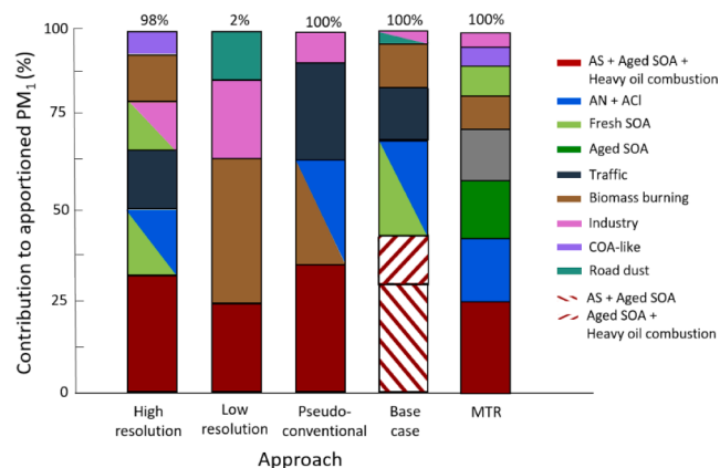
Fig. 8. Summary of source apportionment results of all input PMF datasets. Percentages at the top of each bar represent the fraction of the PM 1 mass that each data subset contains depending on the species it contains. In the base case the split of factors is represented as wefted bars.
