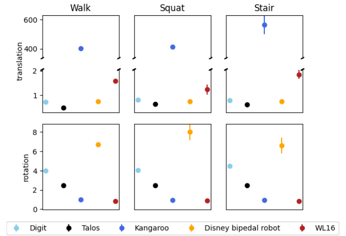
Fig. 4. Velocity manipulability of the foot, in translation (TM, top) and rotation (RM, bottom)
