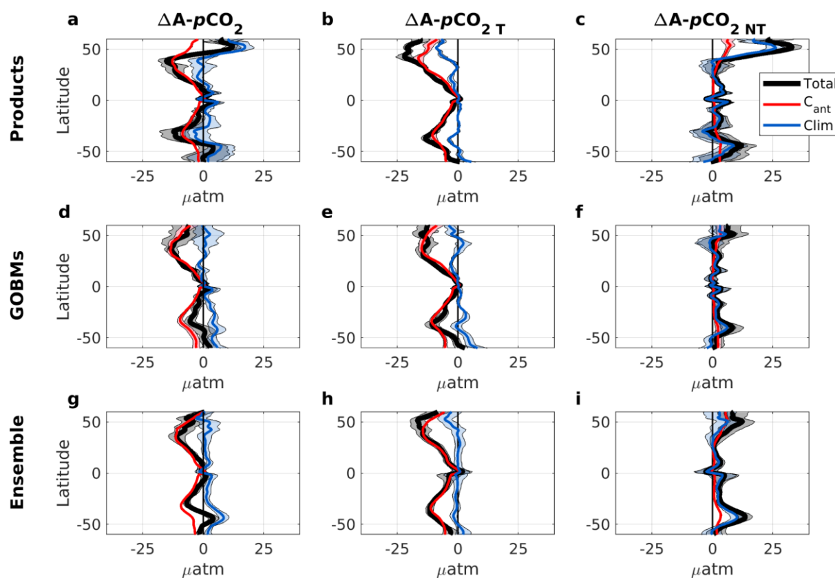
Fig. 10: Mean change in the seasonal cycle amplitude (winter minus summer) of pCO_2 and its thermal (T) and nonthermal (NT) components from the period 1985-1989 to the period 2014-2018. Changes are broken down into the total change and the portion of the change attributed to the accumulation of anthropogenic carbon ( C_{\text{ant}} ) versus climate (Clim: changes to the ocean physical or biogeochemical state caused by anthropogenic climate change). The top, middle, and bottom rows show the ensemble mean results for the three pCO_2 products, the eleven GOBMs listed in Table 3 , and the CESM2 large ensemble, respectively. Shading reflects the standard deviation across the pCO_2 products, GOBMs, and ensemble members. Seasons are defined as JFM and JAS.
