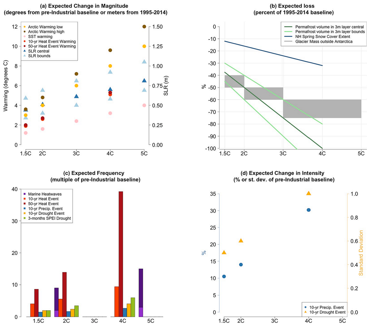
Fig. 2. For all metrics whose future changes were found to have a quantitative relation with GSAT warming we represent such changes for discrete GWLs (1.5 °C, 2 °C, 3 °C, 4 °C and 5 °C, or a subset of them depending on the availability of the corresponding estimates).
