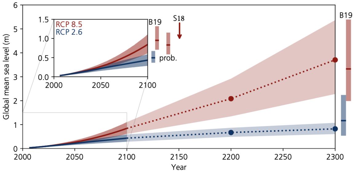
Figure 4.2: Projected sea-level rise until 2300. The inset shows an assessment of the likely range of the projections for RCP2.6 and RCP8.5 up to 2100 (medium confidence). Projections for longer time scales are highly uncertain but a range is provided (4.2.3.6). For context, results are shown from other estimation approaches in 2100. The two sets of two bars labelled B19 are from an expert elicitation for the Antarctic component (Bamber et al., 2019), and reflect the likely range for a 2 and 5°C temperature warming (low confidence; details section 4.2.3.3.1). The bar labelled “prob.” indicates the likely range of a set of probabilistic projections (4.2.3.2). The arrow indicated by S19 shows the result of an extensive sensitivity experiment with a numerical model for the Antarctic ice sheet combined, like the results from B19 and “prob.”, with results from Church et al. (2013) for the other components of sea level rise. S19 bars also show the likely range.
