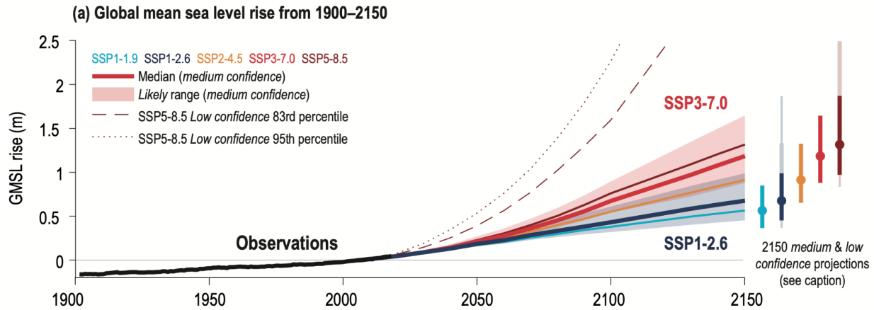
Figure S13. Technical Summary figure (Box TS.4, Fig. 1a) from the IPCC AR6 presenting GMSL time series 37 . Solid lines show median projections. Shaded regions show medium confidence, likely ranges from SSP1-2.6 and SSP3-7.0. Dark bars at right show 2150 likely ranges for all scenarios. Thick/thin lightly shaded bars show 17th-83rd/5th-95th percentile of low confidence projections for SSP1-2.6 and SSP5-8.5 (extending to 4.8/5.4 m for SSP5-8.5).
