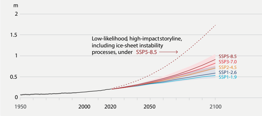
Fig. 3. Different visualizations of global mean sea level (GMSL) projection uncertainty and ambiguity in the IPCC AR6 Working Group 1 report. (a) Tabular presentation of medium confidence* projections for five SSP scenarios and low confidence* projections for SSP5-8.5, presented as Table 9.9 6 . Projections for individual components (first five rows) are for 2100. Values shown are median and likely* ranges, except for the low confidence* projections, where presented ranges are 17th-83rd percentile with no formal likelihood assessed. (b) Projected GMSL change on 100- (blue), 2,000- (green), and 10,000 (magenta) time scales as a function of global surface temperature, relative to 1850-1900, extracted from
