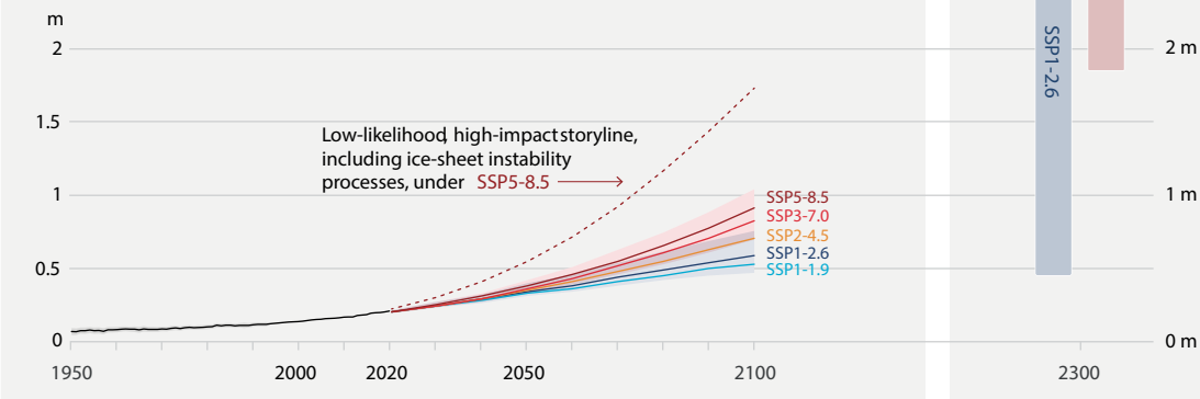
Fig. 3. Different visualizations of global mean sea level (GMSL) projection uncertainty and ambiguity in the IPCC AR6 Working Group 1 report. (a) Tabular presentation of medium confidence* projections for five SSP scenarios and low confidence* projections for SSP5-8.5, presented as Table 9.9 6 . Projections for individual components (first five rows) are for 2100. Values shown are median and likely* ranges, except for the low confidence* projections, where presented ranges are 17th-83rd percentile with no formal likelihood assessed. (b) Projected GMSL change on 100- (blue), 2,000- (green), and 10,000 (magenta) time scales as a function of global surface temperature, relative to 1850-1900, extracted from
