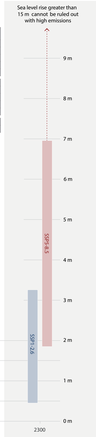
Fig. 3. Different visualizations of global mean sea level (GMSL) projection uncertainty and ambiguity in the IPCC AR6 Working Group 1 report. (a) Tabular presentation of medium confidence* projections for five SSP scenarios and low confidence* projections for SSP5-8.5, presented as Table 9.9 6 . Projections for individual components (first five rows) are for 2100. Values shown are median and likely* ranges, except for the low confidence* projections, where presented ranges are 17th-83rd percentile with no formal likelihood assessed. (b) Projected GMSL change on 100- (blue), 2,000- (green), and 10,000 (magenta) time scales as a function of global surface temperature, relative to 1850-1900, extracted from
