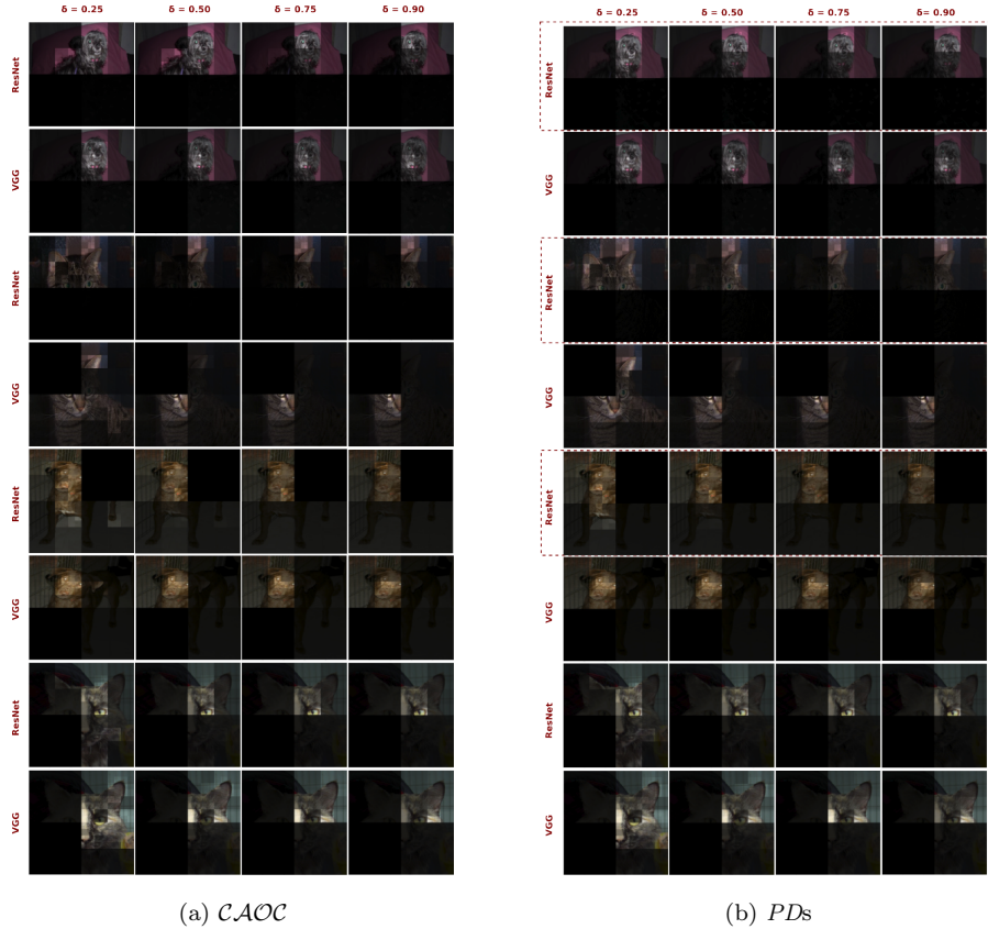
Figure 5: Ms-IV visualizations using \mathcal{CAOC} metric to measure patch importance for image samples (two dogs and two cats) using VGG16/ResNet-18 (explanations in the text).
