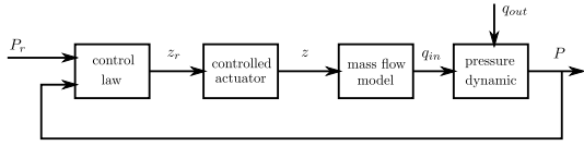
Fig. 2: Block diagram of the feedback control system.
