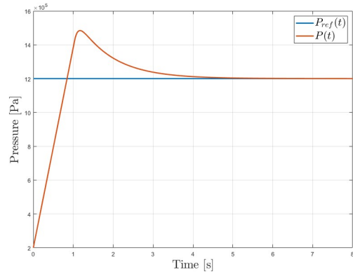
Fig. 4: Time responses of the output pressure P(t) (in red) and the reference P_{ref} (in blue).
