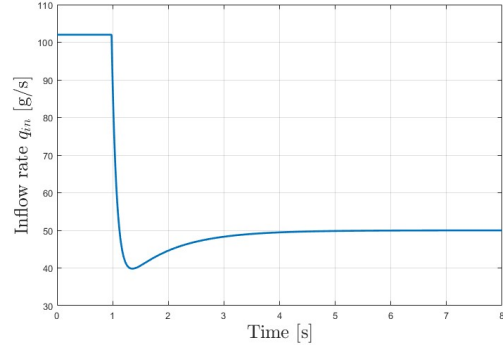
Fig. 5: Time evolution of the (virtual) control input, that is the inflow rate q_{int}(t) .
