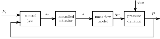
Fig. 2: Block diagram of the feedback control system.
