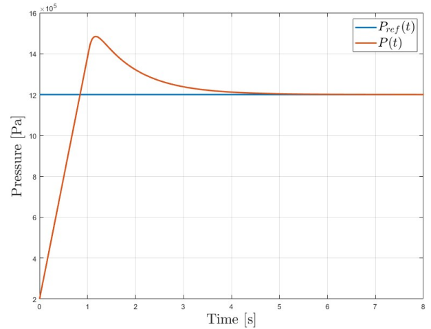
Fig. 9. Time responses of the output pressure P(t) (in ref) and the reference P_{ref} (in blue).
