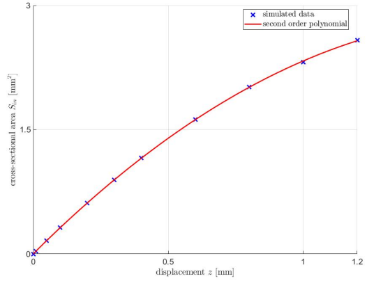
Fig. 4. Opening area at the bottleneck w.r.t. the needle position of the actuator.
