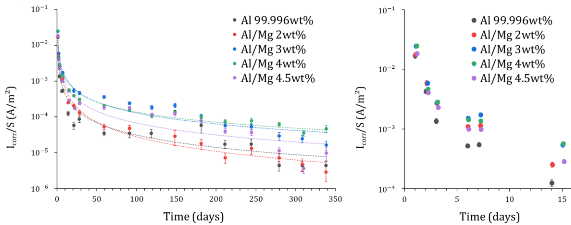
Figure 12. Evolution of the corrosion current I_{corr}/S derived from fitting the EIS spectra for Al and Al/Mg alloys embedded in MKP mortar, normalized by the surface of electrode S.
