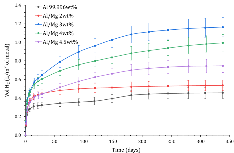
Figure 13. Variation with time of the normalized H_2 production calculated by EIS as a function of the alloy grade ( P = 1 \text{ atm} , T = 25 \text{ }^\circ\text{C} ).
