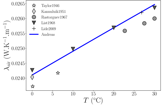
Figure 2: Temperature effect on thermal conductivity of air. Experimental data obtained by hot wire measurements extracted from Taylor and Johnston [38] ( \star ), Kanmulluik and Carman [39] ( \diamond ), Rastorguev and Geller [40] ( \circ ) and reference data extracted from List [24] ( \nabla ) and Lide [23] ( + ). Deep blue curve is equation (9).
