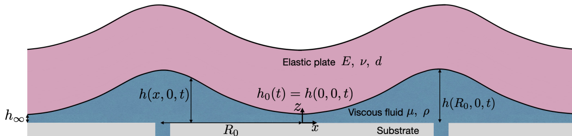
FIG. 1: A cross sectional schematic ( y = 0 ) of the studied system. Two identical pockets filled with a viscous fluid of viscosity \mu and density \rho are created by injecting prescribed fluid volumes beneath an elastic plate. The elastic plate has a Young modulus E , a Poisson ratio \nu , and a thickness d . After the fluid injection is stopped, each blister spreads until reaching a radius R_0 when they meet, which is defined as time t = 0 . The fluid height profile is h(x, y, t) , while h_0(t) = h(0, 0, t) is the bridge height, h_i = h(\pm R_0, 0, 0) is the initial blister height, and r(t) is the half-width of the bridge along the y -axis.
