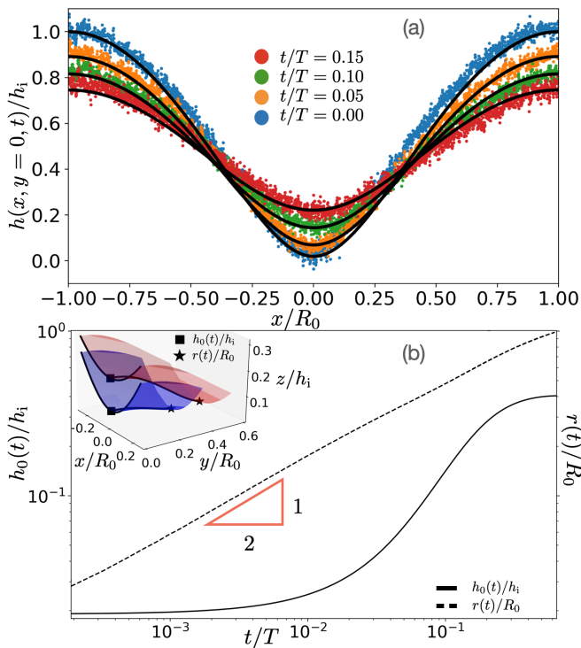
FIG. 2: (a) Dimensionless cross-sectional height profiles h(x, y = 0, t)/h_i , at different dimensionless times t/T , from an experiment with \mu = 0.5 Pa s and h_i = 2.55 mm, and from the numerical solutions (solid lines) of Eq. (1) with N = 59 and h_\infty/h_i = 0.019 . (b) Dimensionless height h_0(t)/h_i , and half-width r(t)/R_0 of the bridge, extracted from the numerical solutions of Eq. (1). Inset: Dimensionless height profiles h(x, y, t)/h_i from the numerical simulation of Eq. (1), at dimensionless times t/T = 0.11 (blue) and t/T = 0.19 (red). The bridge half-width r(t) and height h_0(t) are indicated by the star and square markers, respectively.
