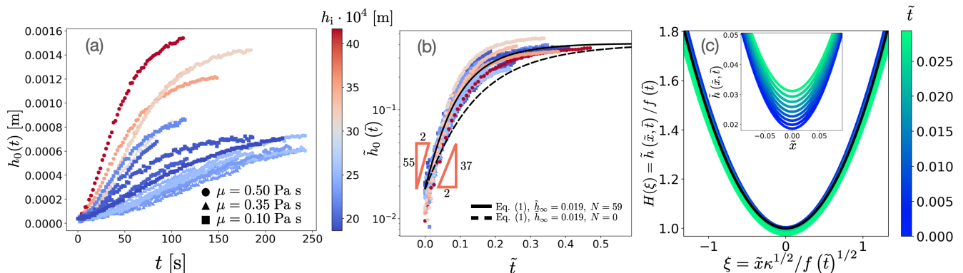
FIG. 3: (a) Experimental bridge height h_0(t) for different viscosities \mu \in [0.1, 0.35, 0.5] Pa s and blister peak heights h_i \in [1.9 - 4.2] \cdot 10^{-3} m. (b) Experimental dimensionless bridge height \tilde{h}_0(\tilde{t}) = h_0(\tilde{t})/h_i as a function of dimensionless time \tilde{t} = t/T . The solid and dashed lines represent the numerical solutions of Eq. (1) for N = 59 and N = 0 , respectively, and with \tilde{h}_\infty = 0.019 . The short-time behaviour for N = 59 is well described by \tilde{h}_0(\tilde{t}) = \tilde{h}_0(0) \exp(27.5\tilde{t}) ; while for N = 0 it follows \tilde{h}_0(\tilde{t}) = \tilde{h}_0(0) \exp(18.5\tilde{t}) . (c) Inset: The height profiles \tilde{h}(\tilde{x}, \tilde{y} = 0, \tilde{t}) (noted \tilde{h}(\tilde{x}, \tilde{t}) ) from the short-time numerical solution of Eq. (1) for N = 0 and \tilde{h}_\infty = 0.019 . Main: Self-similar representation of the height profiles ( \tilde{y} = 0 ) from Eq. (1) shown in the inset. Here, we used f(\tilde{t}) = 1.9 \cdot 10^{-3} \exp(18.5\tilde{t}) and \kappa = 8 . The black solid line is the numerical solution of Eq. (5) with \kappa = 8 and \alpha = 0.0181 .
