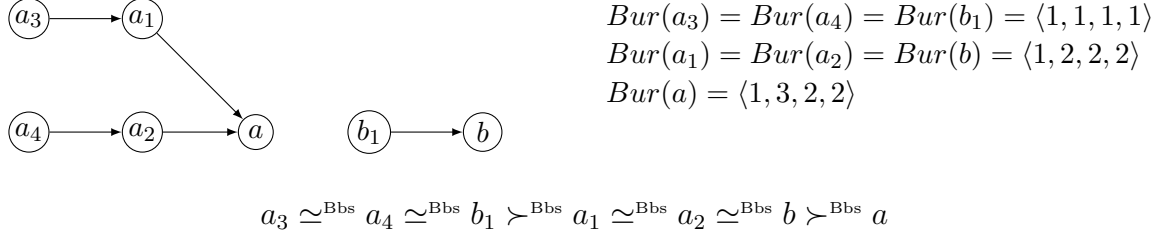
Fig. A.4. The burden-based semantics falsifies the property AvsFD.
