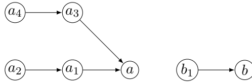
Fig. A.23. The iterated graded defense semantics falsifies the property AvsFD.
