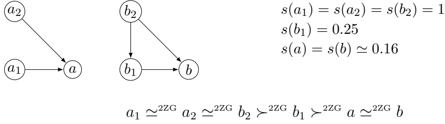
Fig. A.14. The ranking-based semantics 2ZG falsifies the property DP.
