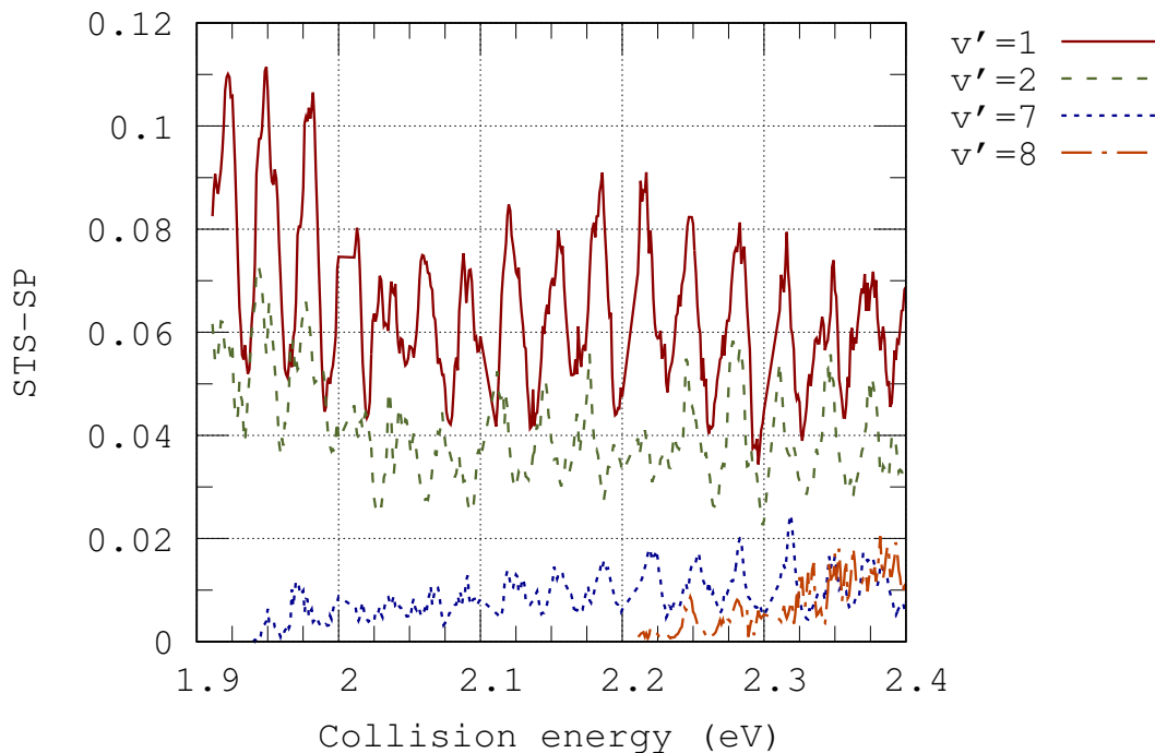
Figure 5: Vibrational state-to-state resolved scattering probabilities for inelastic activation processes of \text{o-}^{14}\text{N}^{14}\text{N} in its ground rovibrational state by ^{15}\text{N} : the 5 + \text{o}44(v = 0, j = 0) \rightarrow 5 + \text{o}44(v', \text{all } j' \text{ even } \neq (0, 0)) processes, as a function of collision energy in eV.
