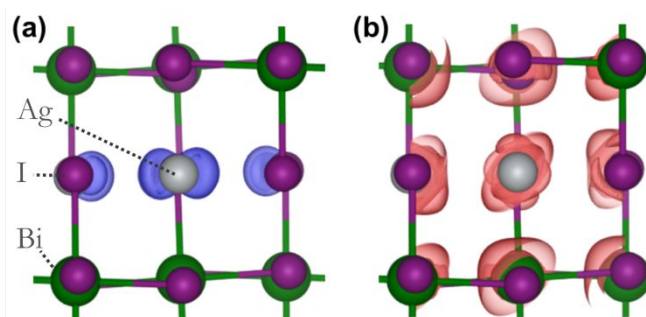
Fig. 3 Localized density of states at the (a) VBM and (b) CBM computed for \text{AgBiI}_4 with a Imma model crystallographic structure. The grey, green, and purple spheres indicate Ag, Bi, and I atoms respectively.
