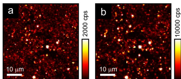
Fig. 4. Multiphoton absorption-based luminescence maps of the drop-casted \text{AgBiI}_4 NCs at spectral regions corresponding to (a) 300 to 400 nm, and (b) 400 nm to 650 nm. The input polarization is along the vertical. The collected signals are not polarization-analyzed. The maps are plotted at different scales (in terms of signal counts per second or cps) for emphasis. The resolution of the maps is 100 × 100 pixels.
