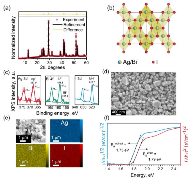
Fig. 2 (a) Experimental (open circles) and refined (solid line) profiles and their difference (yellow line) obtained after the full-pattern Rietveld refinement of the XRD patterns of \text{AgBiI}_4 NC film. (b) The refined crystal structure of \text{AgBiI}_4 . (c) XPS core-level spectra of Ag 3d, Bi 4f, and I 3d. (d) High magnification SEM image of the \text{AgBiI}_4 NCs. (e) SEM-EDS color maps showing the distribution of Ag, Bi, and I in the \text{AgBiI}_4 NC film. (f) Tauc plots of \text{AgBiI}_4 NC film for direct and indirect band gap assumptions.
