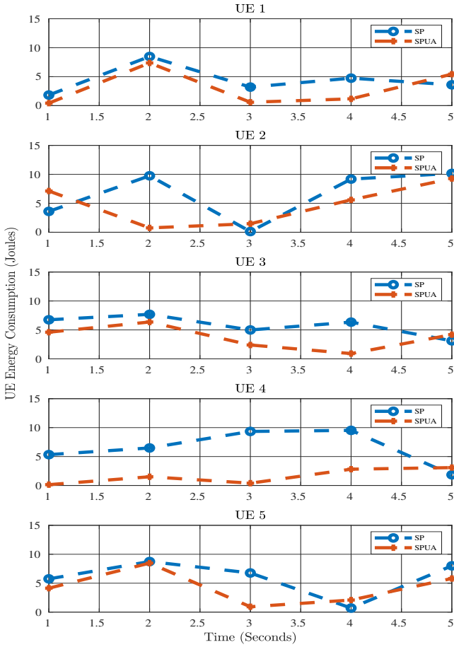
Fig. 2: UE Energy Consumption using SP and SPUA.
