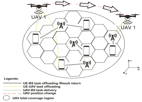
Fig. 1: System Model of the UAV-based MEC system.
