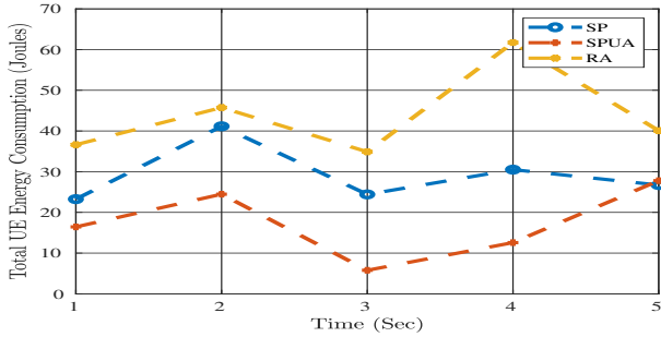
Fig. 3: UE Total Energy Consumption.
