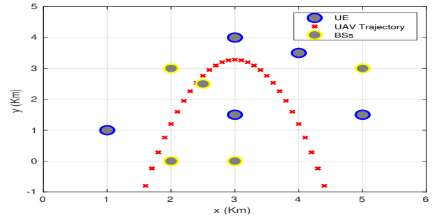
Fig. 4: UAV Trajectory for Energy-Efficient Task Offloading.
