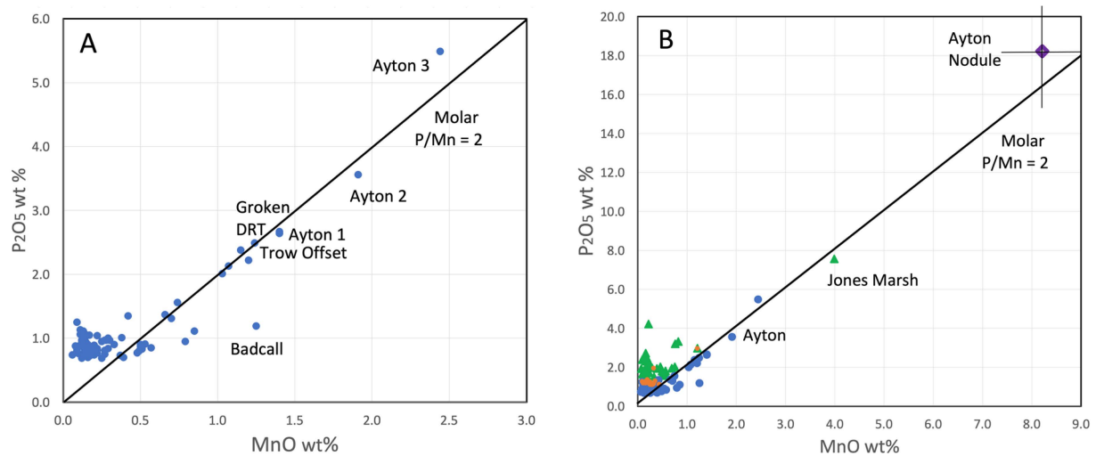
Figure 6. Phosphorus and manganese oxide abundances, APXS analyses. (A) Samples from Knockfarrill Hill member. Ayton 1, 2, and 3 were used to deconvolve the nodule composition, in Table 2. The Badcall sample is enriched in Mn but not P, showing that the Knockfarrill Hill member experienced multiple styles of chemical alteration [8]. (B) Samples from the whole Murray Fm, and the deconvolved composition of the Ayton nodules [8,40]; blue = Knockfarrill Hill; green = Vera Rubin Ridge; orange = other Glen Torridon. The Jones_Marsh sample, a nodular surface, is richer in Mn and P than the Ayton samples and has molar P/Mn = 2. Uncertainty bars on the Ayton nodule deconvolution are 1\sigma .
