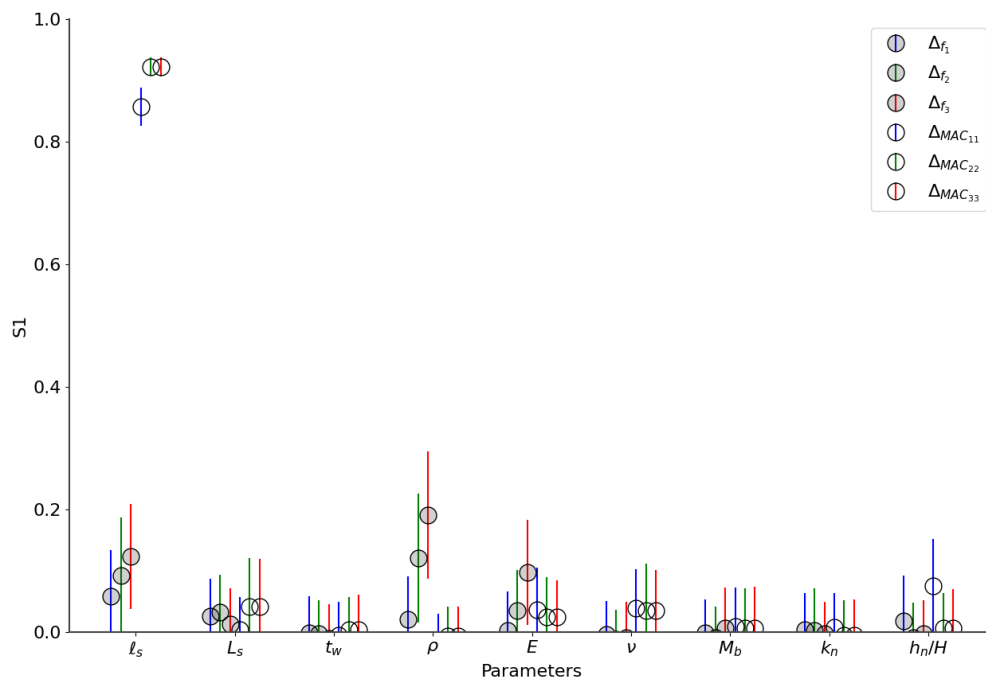
Figure 18. Evaluation of the first-order Sobol indices for the errors regarding the dynamic properties.
