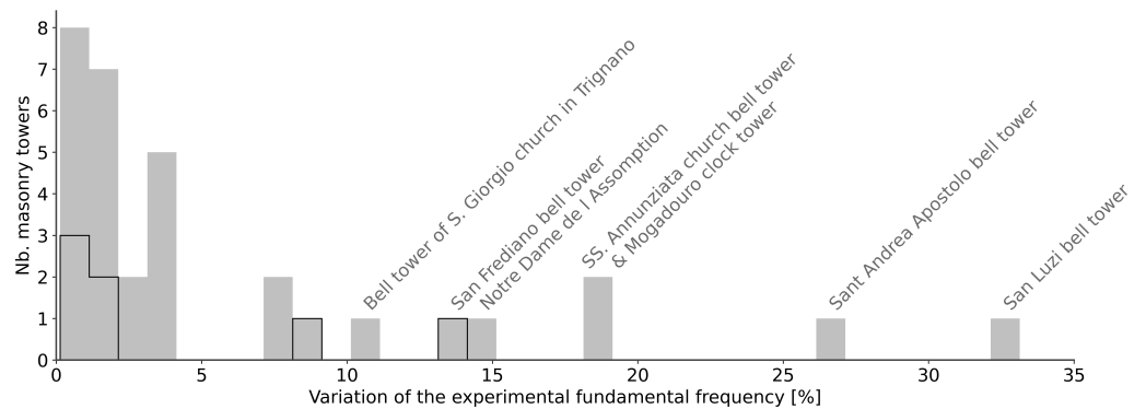
Figure 9. Distribution of variation in the measured fundamental frequency expressed as (f_0^{max} - f_0^{min})/f_0^{min} , i.e., the maximum difference between the minimum and maximum measured fundamental frequency for each instrumented masonry tower. Long SHM (with measurements duration over one day) are plotted with a dark gray edge.
