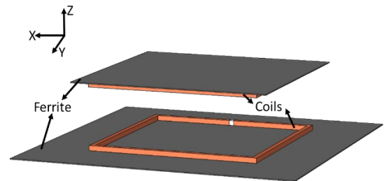
Fig. 1. Initial ferrite volume
