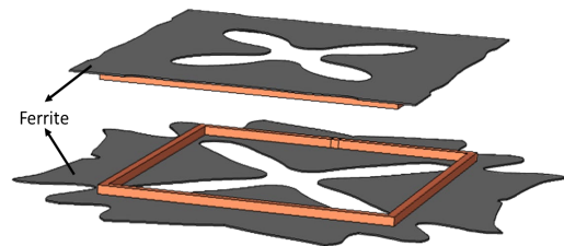
Fig. 2. Structure with 40% reduction of the ferrite volume
