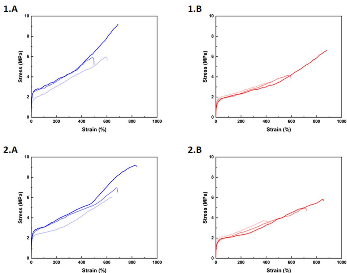
Figure 3. Stress-strain tensile curves for V1 (A) and V1.5 (B): 1. after crosslinking, and 2. after 3 reshaping.
