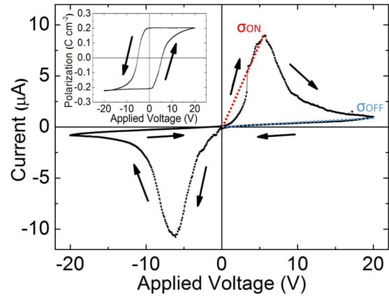
FIG. 2. Typical measured current versus applied voltage for a single crystal at 260 K (for a sawtooth voltage with \omega = 1.2 mHz). For this sample the crystal size is about 200 \mu m \times 400 \mu m \times 1000 \mu m . The peak current density is about 10 mA cm^{-2} . Inset: Corresponding polarization versus applied voltage. Note the colossal value of the polarization. For a typical sample, the integrated charge is of the order of 100 \mu C , which divided by the contact area gives a density of polarization of the order of 0.1 C cm^{-2} .
