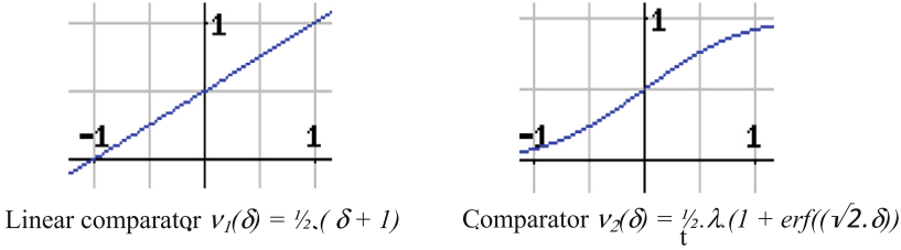
Fig. 7. Graphical representation of two comparators.
