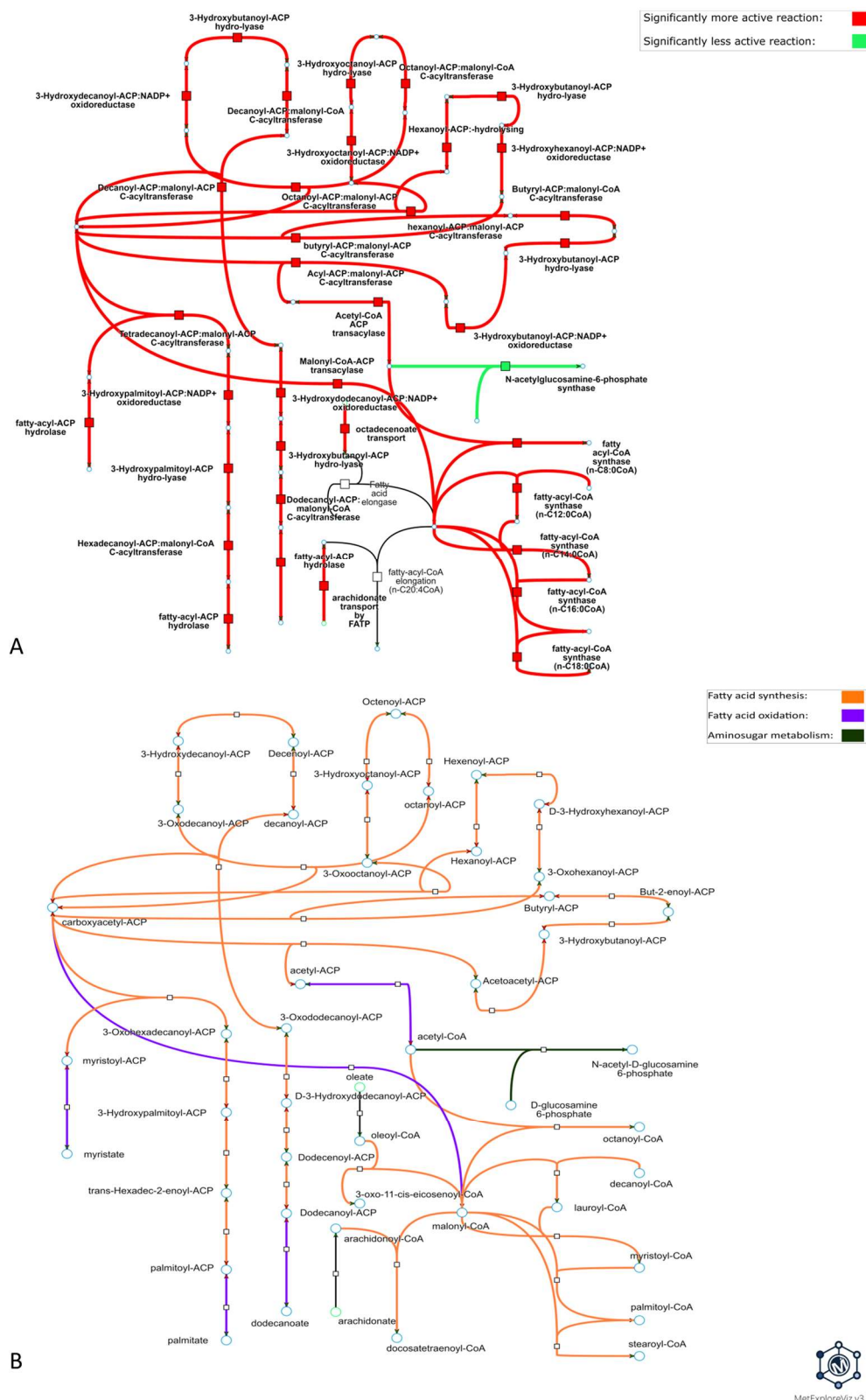
Fig 5. Metabolic visualization of the subnetwork extracted from one the DARs cluster predicted for amiodarone. DARs were predicted by performing condition-specific reconstructions for PHH exposed to 7 \mu M amiodarone for 24h. The visualized subnetwork was computed with DARs from cluster #2, which is the cluster with the highest DARs subnetwork coverage among the clusters identified in the distance matrix (Fig 3A) for this condition. Nodes represented by a square are metabolic reactions and nodes represented by a circle are metabolites. Fig 5A and 5B represent the same subnetwork with the same topology. Links in Fig 5A are highlighted according
