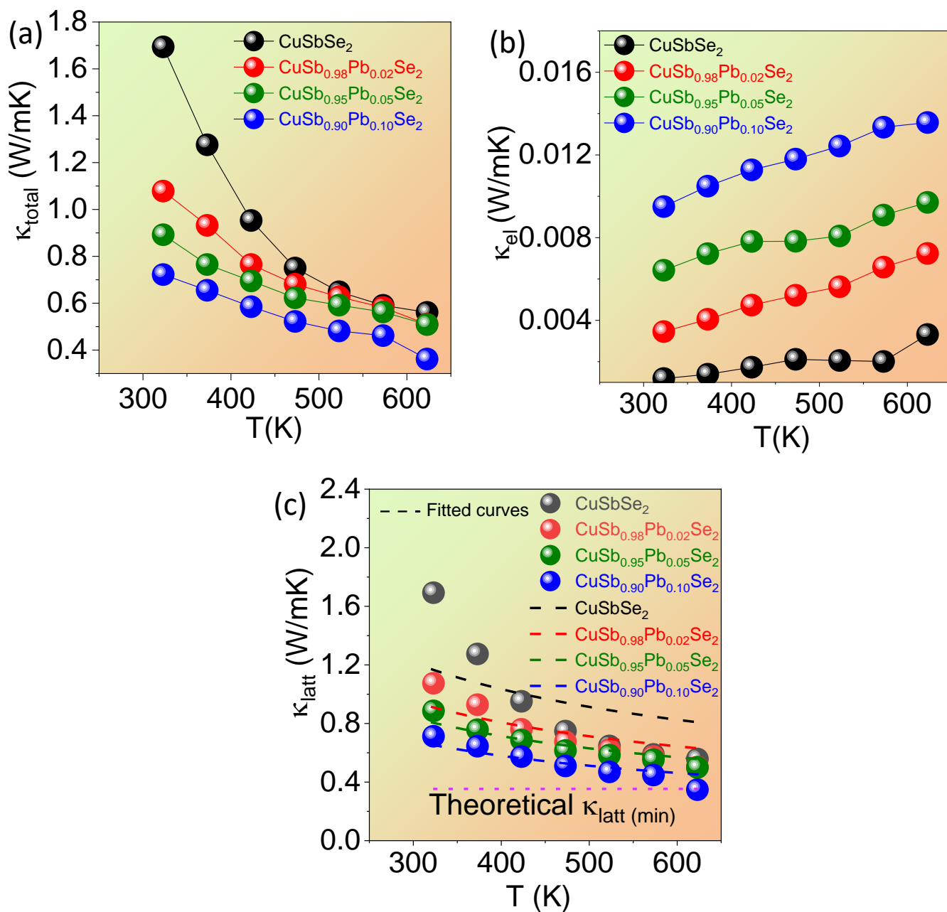
Figure 5. (a) Total thermal conductivity ( \kappa_{\text{total}} ), (b) Electronic thermal conductivity ( \kappa_{\text{el}} ), and (c) Lattice thermal conductivity ( \kappa_{\text{latt}} ) of CuSb 1-x Pb x Se 2 (x = 0-0.10) as a function of temperature.
