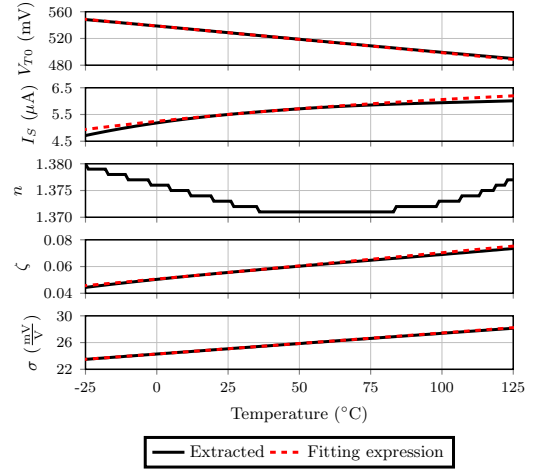
Fig. 6. Temperature variation of the 5 parameters (from top to bottom): V_{T0}(T) , I_S(T) , n , \zeta(T) and \sigma(T) and respective fitting curves for the NMOS transistor from the 0.18 \mu\text{m} CMOS process in Table I.
