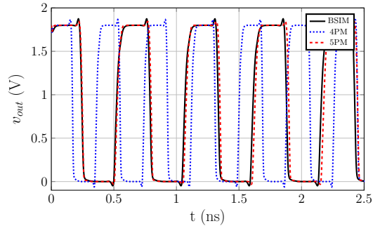
Fig. 10. Output voltage of the simulated 11-stage ring oscillator for 4PM, 5PM and BSIM model
