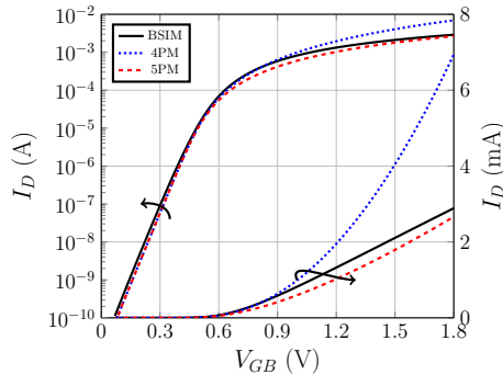
Fig. 3. DC characteristics I_D \times V_{GB} at V_{GB} = V_{DB} of the SVT n-channel MOSFET with W/L = 5 \mu\text{m}/0.18 \mu\text{m} from a 0.18 \mu\text{m} CMOS process.
