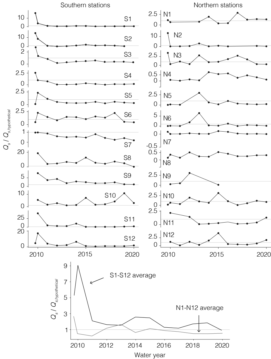
Figure 7. Q_s/Q_{s,hypothetical} after Morakot at the focus gauging stations (Figure 1). Horizontal gray lines indicate Q_s/Q_{s,hypothetical} = 1 . Note different y-axis extents in the individual station plots. At all but one of the southern focus stations, Q_s was elevated above Q_{s,hypothetical} at some point in the first two years after Morakot. By contrast, at seven the twelve northern stations, Q_s does not exceed Q_{s,hypothetical} at any time in the first two years after Morakot. The bottom panel shows the average Q_s/Q_{s,hypothetical} ratios across the southern and northern focus stations. This shows that Q_s at the southern stations was, on average, substantially higher than Q_{s,hypothetical} in the first two years after Morakot, but not at the northern stations.
