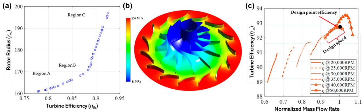
Figure 10. ANN modelled supercritical CO 2 turbine efficiencies. (a) Optimized efficiencies for a range of rotor radii calculated from a multi-objective genetic algorithm optimization of an ANN model. (b) Multiphysics simulation of pressure distribution of the on the surface of the optimized hub/rotor geometry. (c) Simulated off-design performance of the optimized turbine geometry. Adapted with permission from Ref. [214]. Copyright 2021 MDPI.
