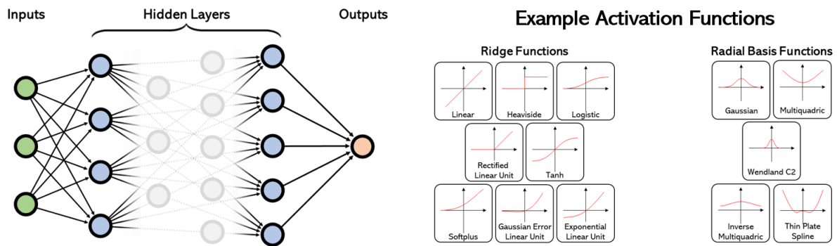
Figure 3. Typical representation of an artificial neural network (ANN). A given set of inputs (green circles) are fed into a network of nodes organized in layers (blue circles) before calculating an output (orange circle). Each node within the hidden layer represents a mathematical ‘activation’ function. Typically, these are either ridge or radial basis functions. Examples of activation functions are given to the right of the main diagram. The exact forms and weights used in the functions within the hidden layers are determined during training.
