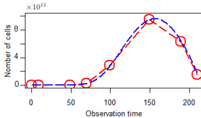
Fig. 11. Susceptible cells dynamics (red) and its estimated (blue) according to Table 2.
