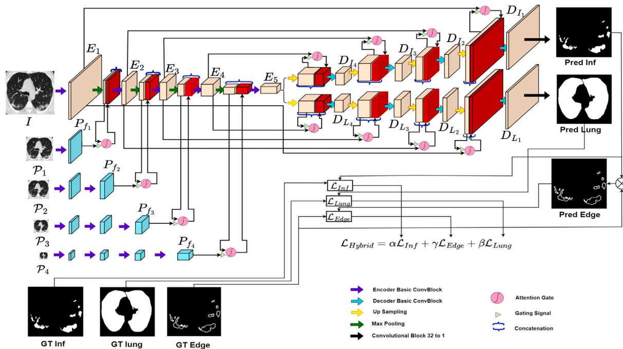
Fig. 3. Our proposed Pyramid PDEAtt-Unet. Both PDEAtt-Unet and PDEAtt-Unet have identical architecture. However, PDEAtt-Unet exploits loss function denoted as Edge loss.
